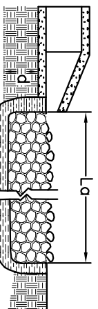
SECTION A-A FILTER BLANKET
