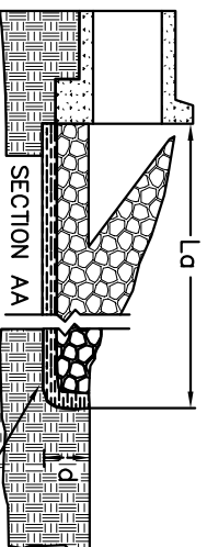
SECTION AA FILTER BLANKET
