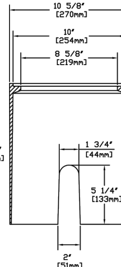
FRAME SECTION
