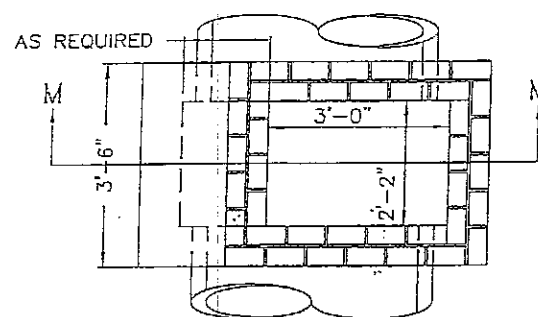
PLAN OVER-LENGTH
