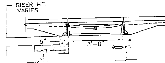
OVER-LENGTH
