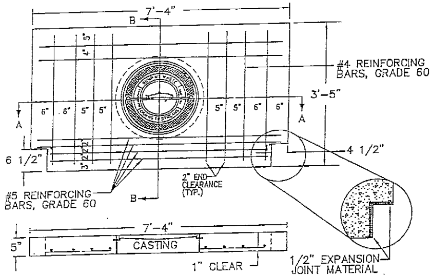
A-A OVER-LENGTH
