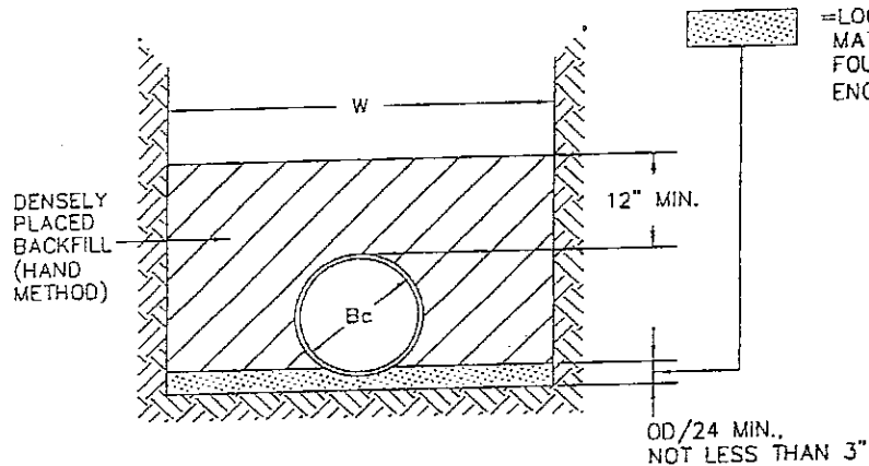
CONTINUOUS BEARING SUPPORT MODIFIED CLASS D
