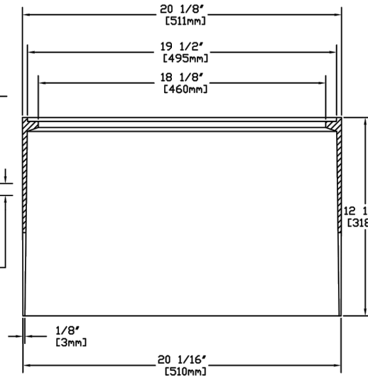
FRAME SECTION
