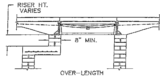
DETAIL SHOWING METHOD OF RISER CONSTRUCTION
