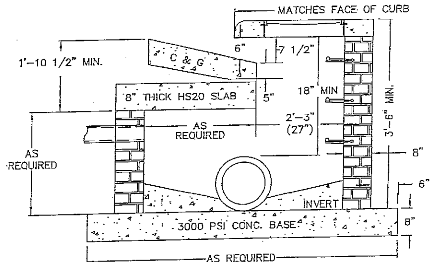
B-B OVER-WIDTH
