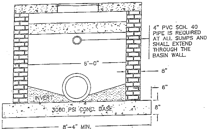
A-A OVER-LENGTH
